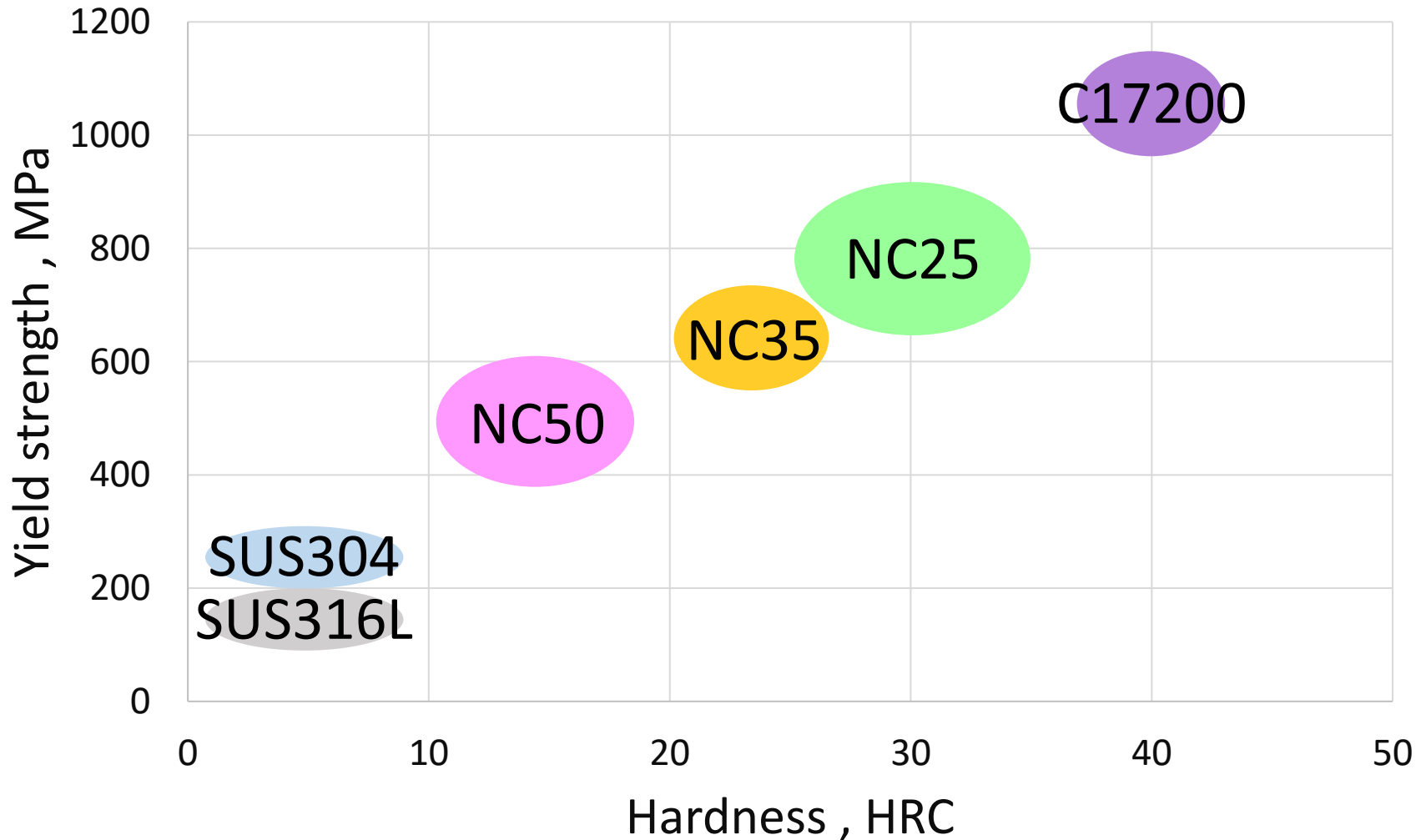
Fig. Relationship between yield strength and hardness
